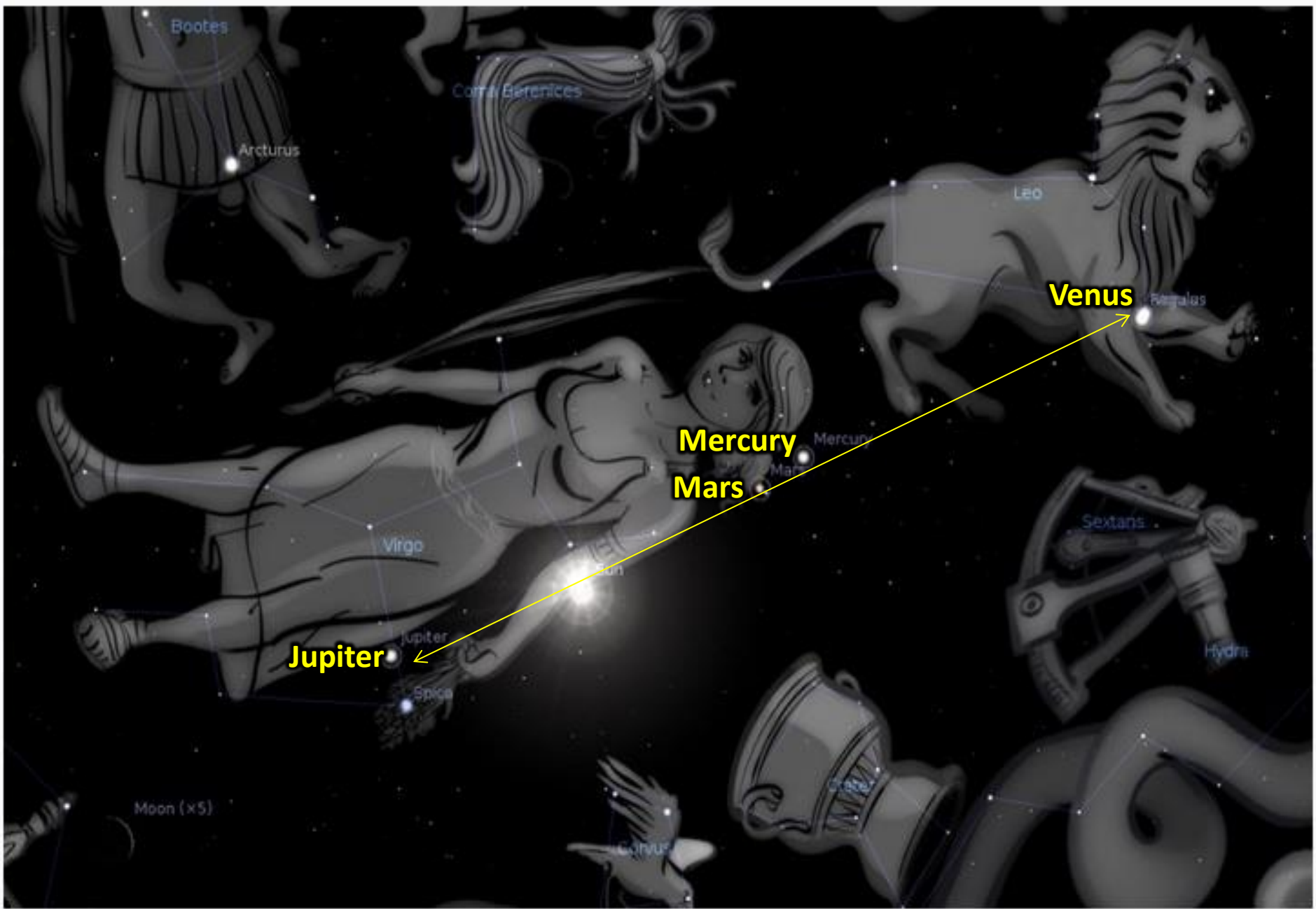
The constellation Virgo on September 14, 1056. Venus and the star Regulus in Leo are very close to one another. 29
