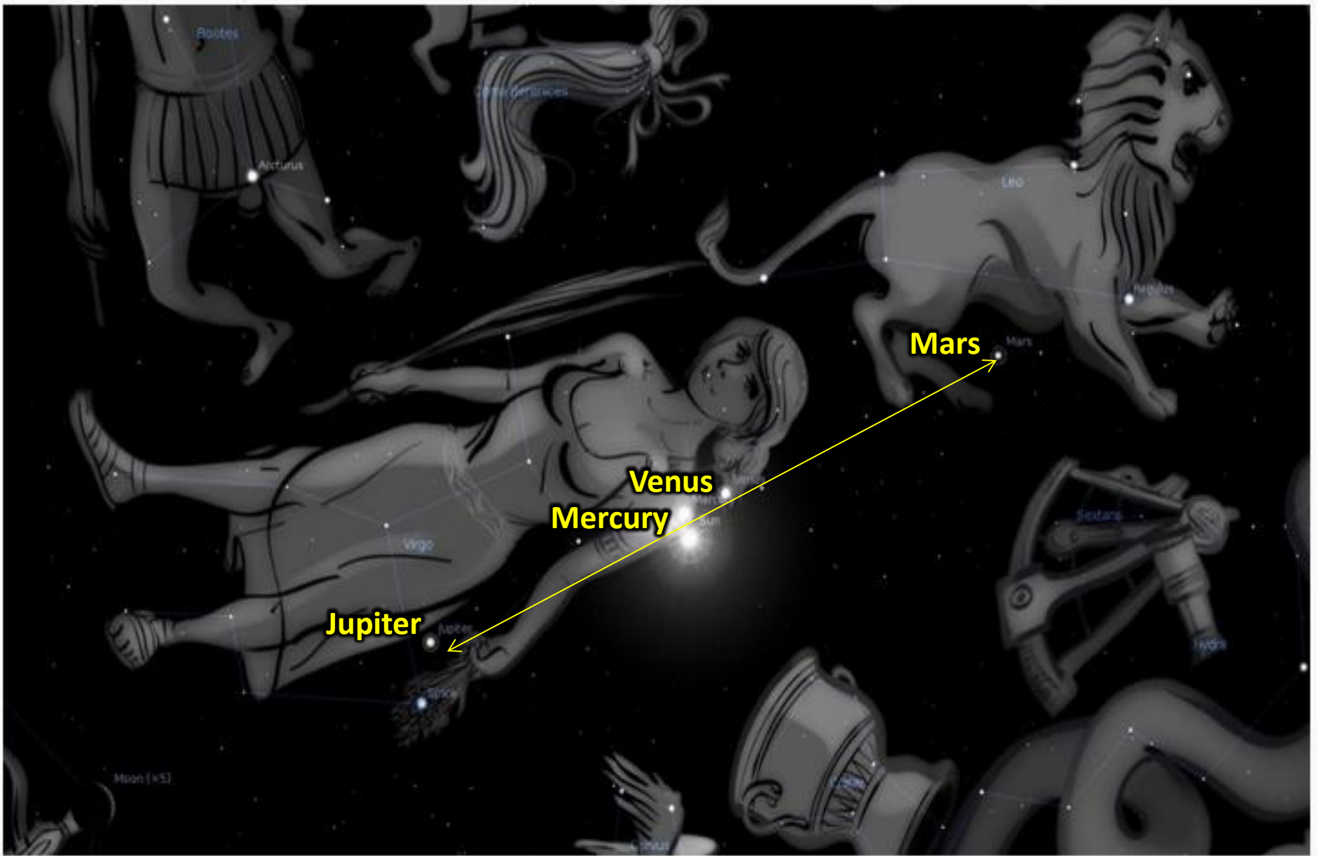
The constellation Virgo on September 24, 1827, according to Stellarium. In this and the images below, the moon's size is exaggerated for visibility. Click any image to enlarge it.
