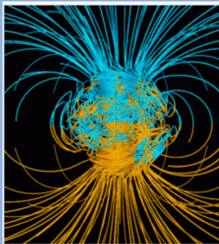
Computer simulation of the Earth's field in a normal period between reversals. [1] The lines represent magnetic field lines, blue when the field points towards the center and yellow when away. The rotation axis of the Earth is centered and vertical. The dense clusters of lines are within the Earth's core. [2]
